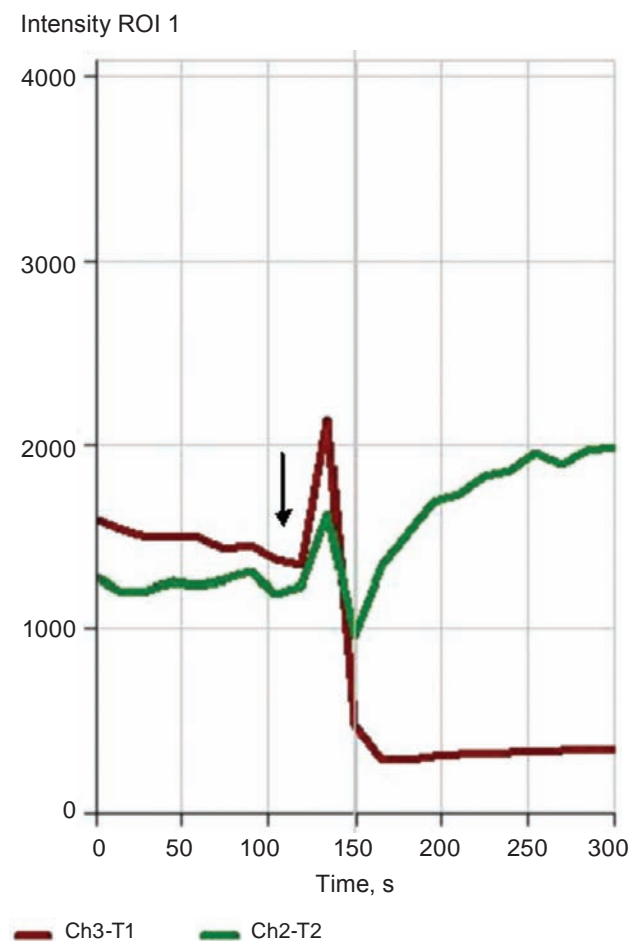
Fig. 5. The fluorescence intensity of potential-sensitive probe TMRM (curve 1) and Ca^{2+} -sensitive probe Fluo-4 AM (curve 2) in rat myometrium cells under the action of calmidazolium ( 10 \mu M ) (the time of addition of calmidazolium marked with an arrow): A – plot of the fluorescence intensities of TMRM and Fluo-4 AM probes with time, (the fluorescence intensities averaged on marked region (ROI)); B – ROI (Region of Interest) (outlined by red circle), which was selected for plotting the fluorescence intensities of TMRM and Fluo-4 AM probes with time
